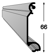
MS123 50MM HD STARTER LATH (0.564 KG/MTR)
