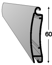
MS140 55MM DBL SKIN LATH (0.54 KG/MTR)
