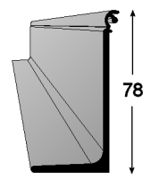
MS130 LD L BOTTOM RAIL (1.006 KG/MTR)
