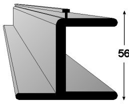
MS141 T BOTTOM RAIL (1.59 KG/MTR)
