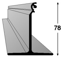
MS128 HD T BOTTOM RAIL (1.41 KG/MTR)
