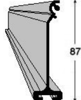
MS152 HD BOTTOM RAIL (0.88 KG/MTR)
