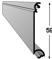
MS129 50MM LD STARTER LATH (0.32 KG/MTR)
