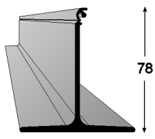
MS132 LD T BOTTOM RAIL (1.364 KG/MTR)
