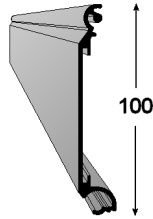
MS124 89MM HD MAIN LATH (0.821 KG/MTR)
