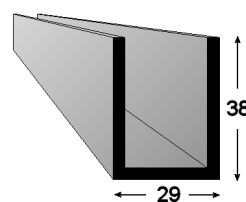
MS131 LD 38MM GUIDE RAIL (0.821 KG/MTR)
