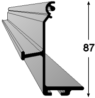
MS125 HD L BOTTOM RAIL (1.206 KG/MTR)
