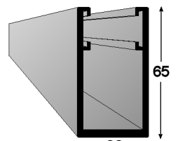
MS127 HD 65MM GUIDE RAIL (1.499 KG/MTR)
