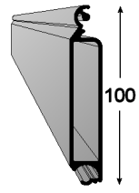
MS150 89MM HD DBL SKIN LATH (1.286 KG/MTR)
