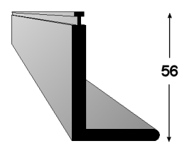
MS142 L BOTTOM RAIL (1.01 KG/MTR)
